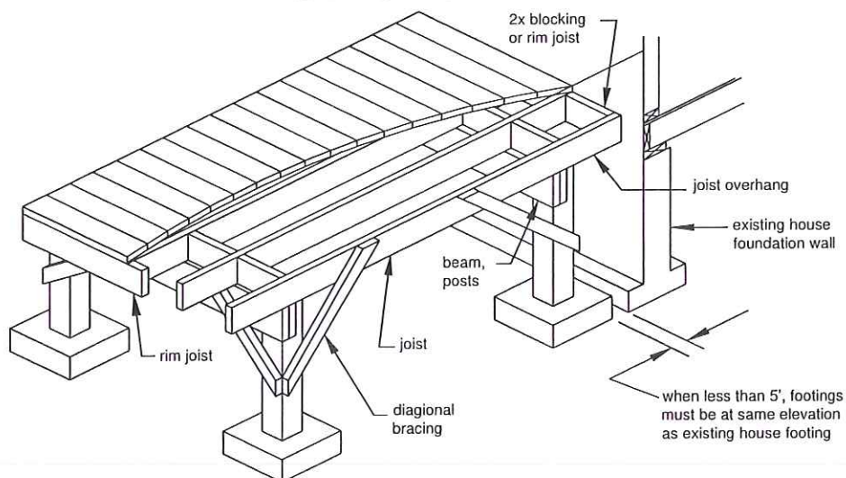
Figure 17 FREE-STANDING DECK
