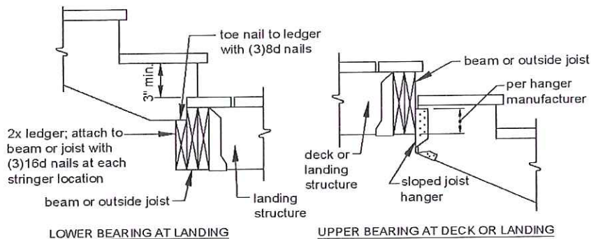
Figure 28 STRINGER BEARING
