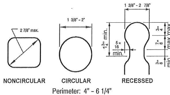
Figure 34 HANDRAIL GRASPABILITY
