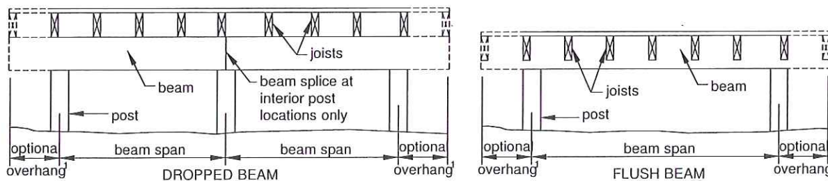
Figure 3 BEAM TYPES
