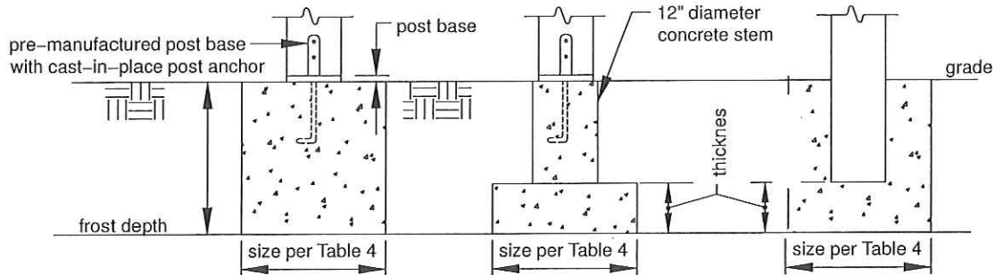
Figure 1 FOOTINGS
