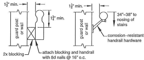
Figure 34 HANDRAIL GRASPABILITY
