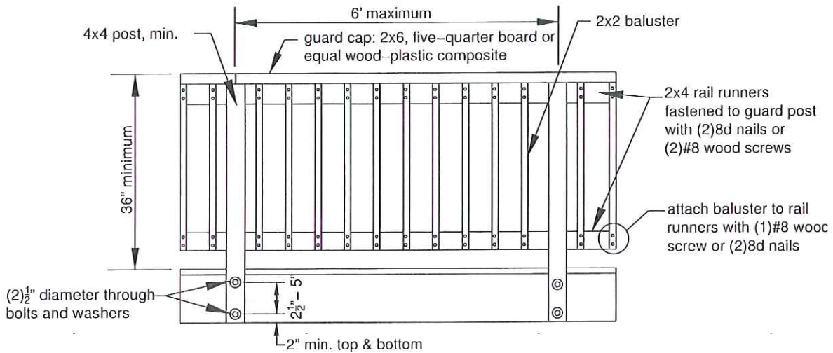
Figure 24 GUARDS
