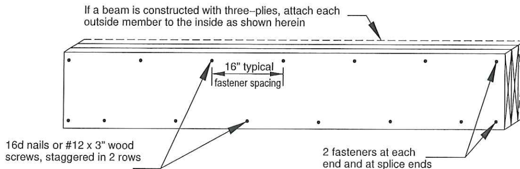
Figure 4 BEAM ASSEMBLY
