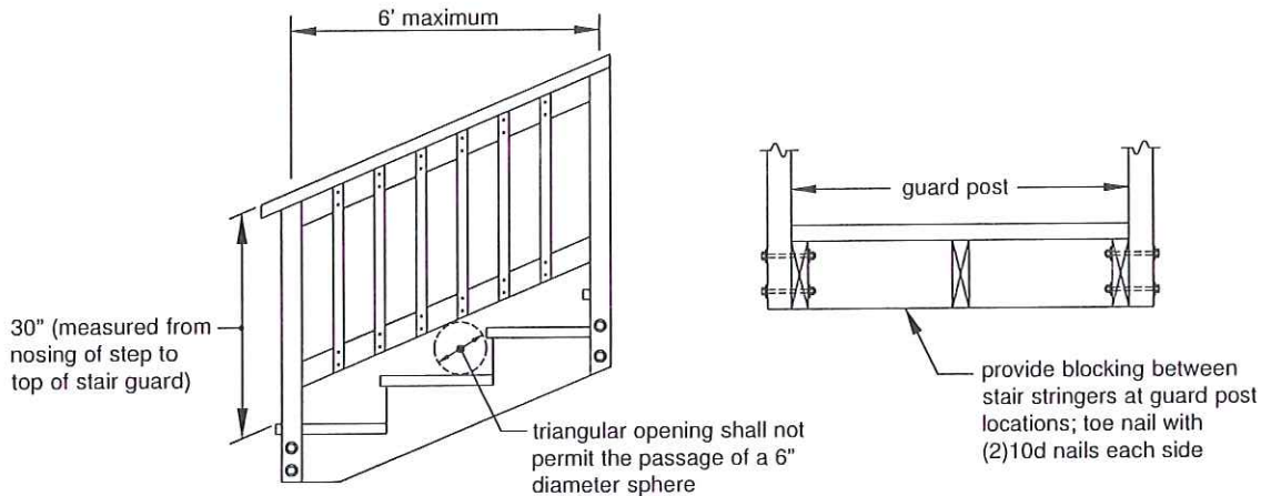
Figure 32 STAIR GUARDS
