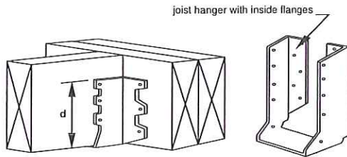
Figure 9 JOIST HANGERS
