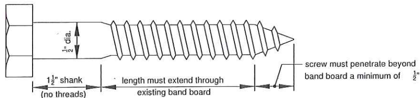
Figure 16 LAG SCREW
