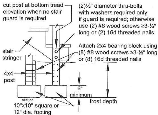
Figure 29 STRINGER BEARING
